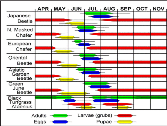
Chart: Cool season white grub life cycle (chart reprinted with permission of Dr. David Shetlar, Entomologist, Ohio State University, www.bugdoc.edu )
