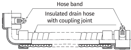
Insulated drain hose with coupling joint x 1 piece (Hose Band x 2 pieces)
