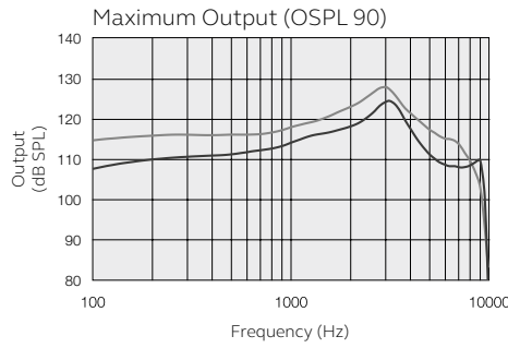
IEC 60118-0: 1983_AMD1:1994 IEC 60118-0:2015 IEC 711 Ear Simulator
